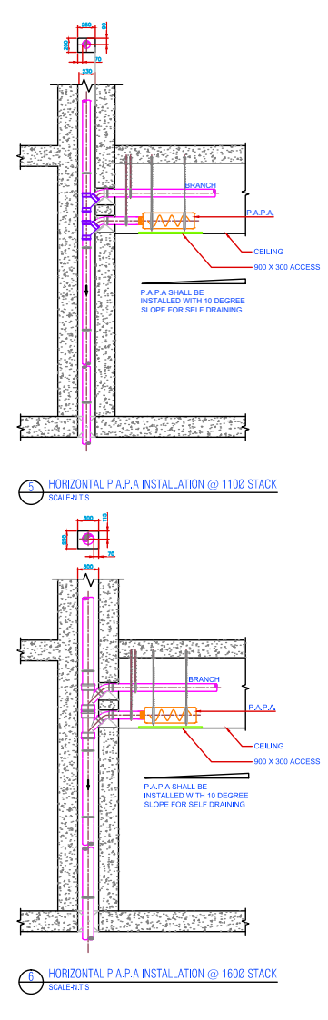
Horizontal floor installation
