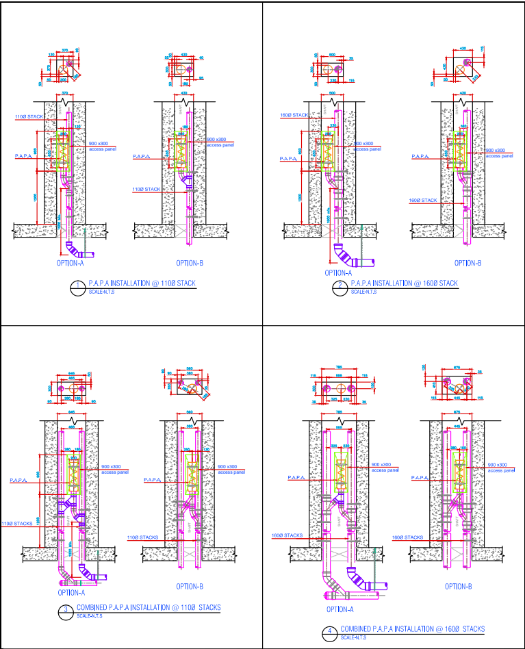
Vertical duct installation
